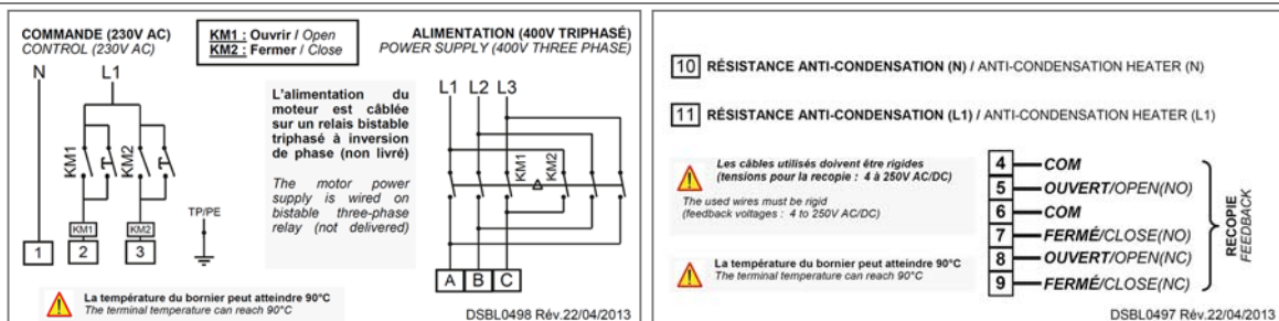
VR/VS 3-phase 400 V
